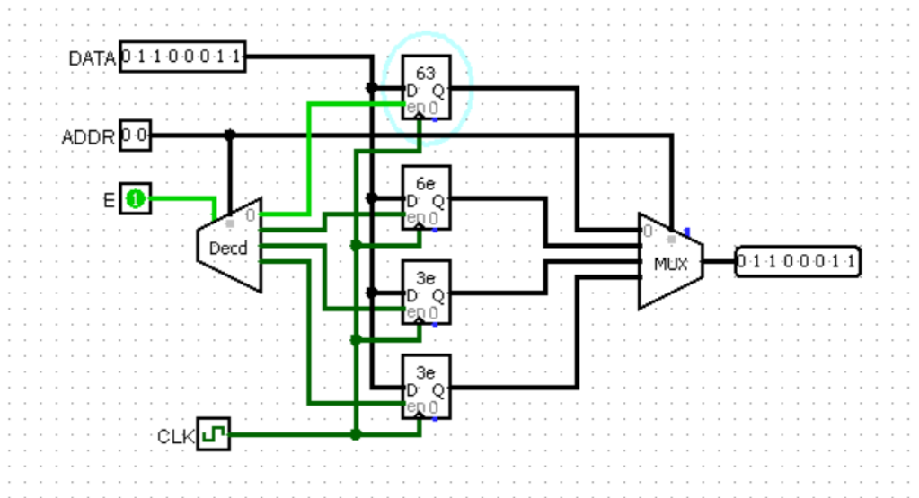
Figure 2: Cấu trúc Register File
